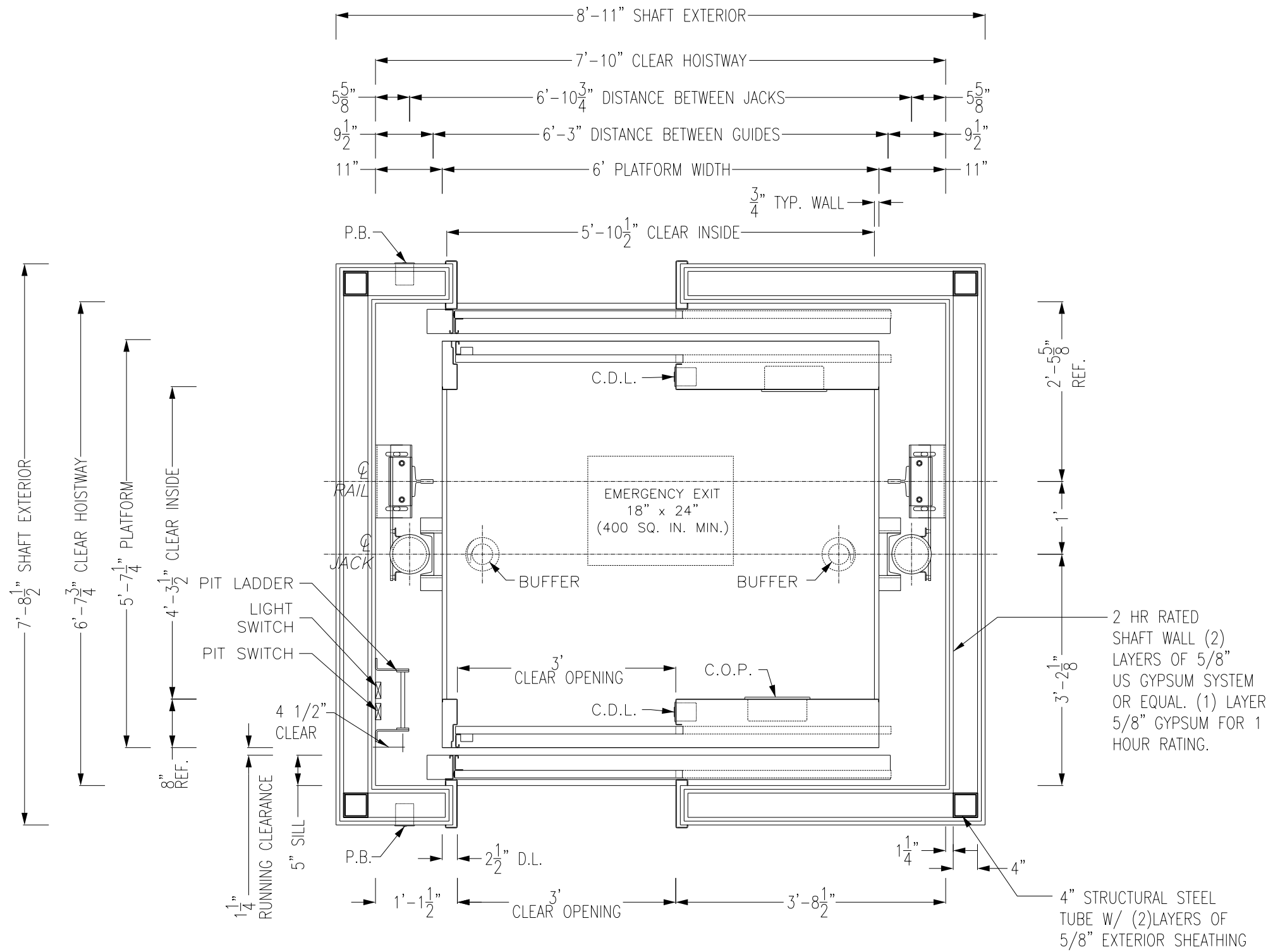
HOISTWAY PLAN
